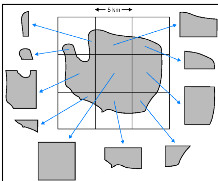
Figure 21: chunking
