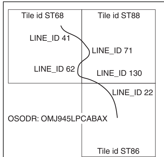
Figure 3.3: Unique identifiers
