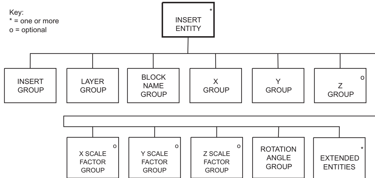
Figure 9.13: Level 3
