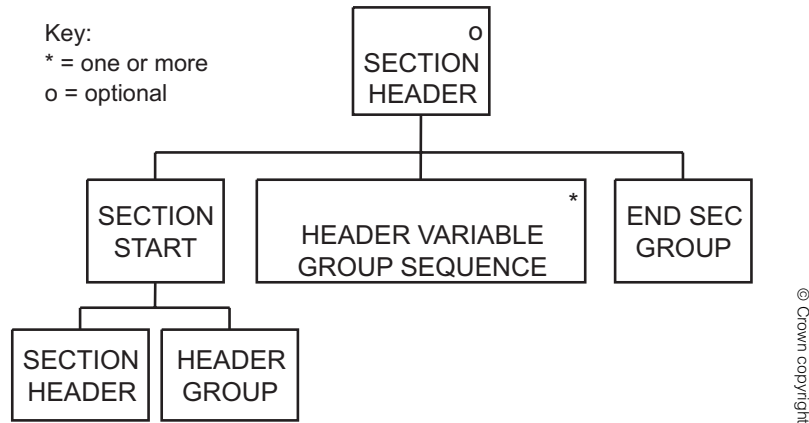
Figure 9.2: Level 2
