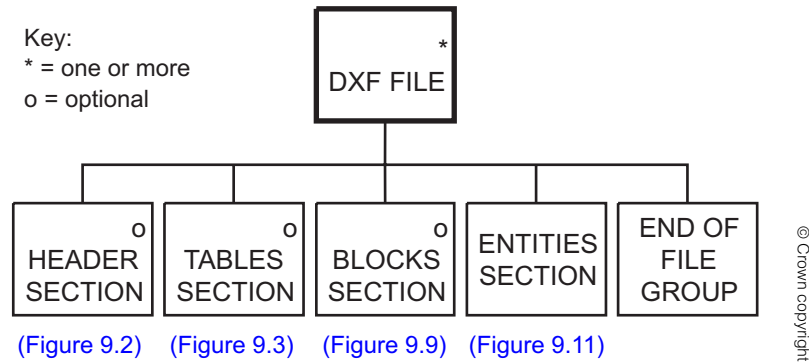
Figure 9.1: Level 1
